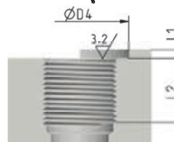
Setting ISO 1179-1
